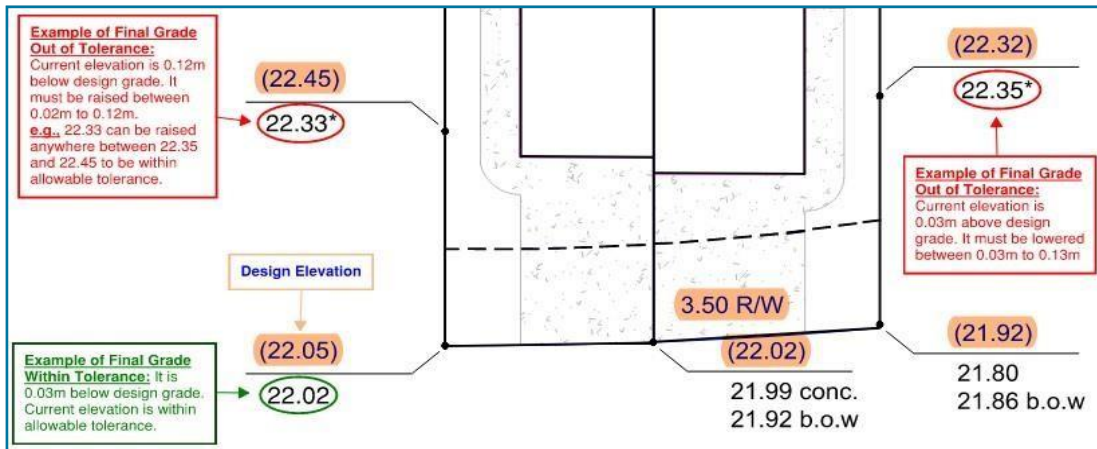
Tolerance Example at Final Grade Stage
